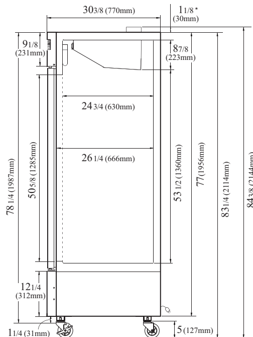
SIDE VIEW *Pressure relief valve
