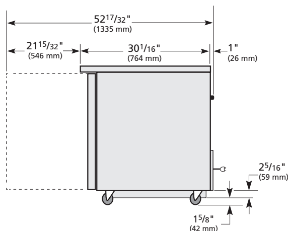
RIGHT VIEW
