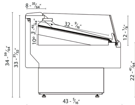
Standard Mounting
