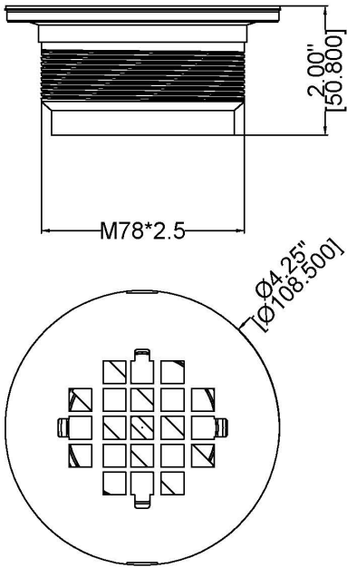
Mop Sink Strainer
