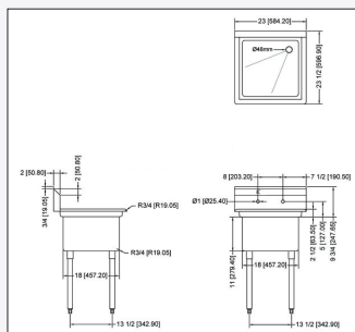
56000-014 no drain board
