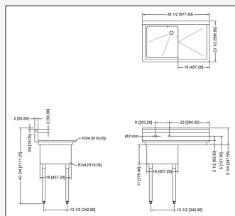
56000-034 right drain board
