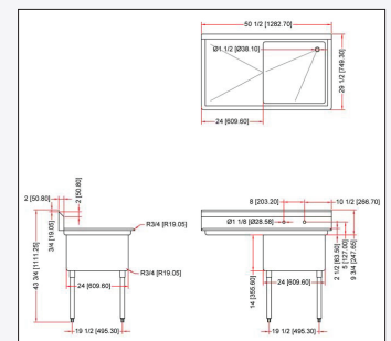
56000-039 left drain board
