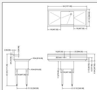
56000-035 two drain boards
