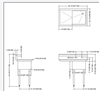
56000-033 left drain board
