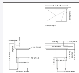
56000-049 left drain board
