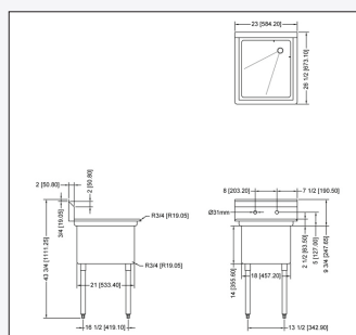
56000-048 no drain board
