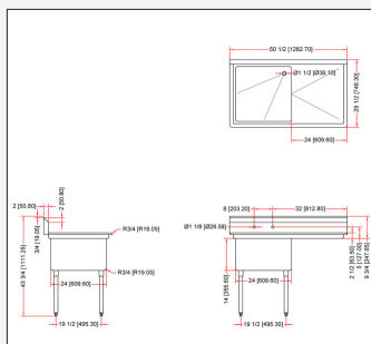
56000-040 right drain board
