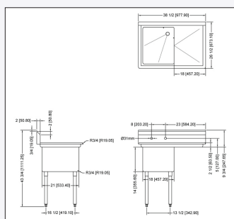
56000-050 right drain board
