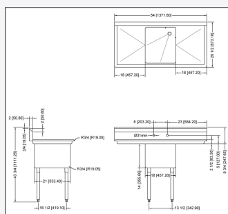
56000-051 two drain boards
