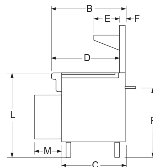
Ranges with Cabinet Base
