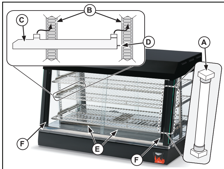
Figure 5. Doors, Light, Shelf Brackets and Shelf Support.
