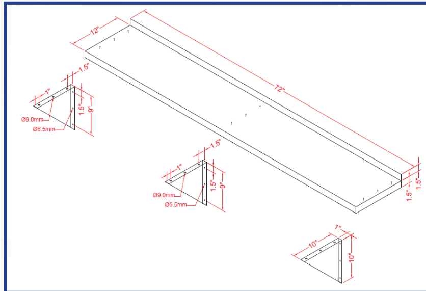
12" x 72" Wall Shelf
