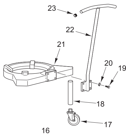
BOWL TRUCK
